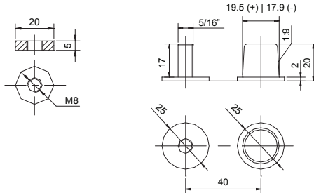
Terminal (M8)
